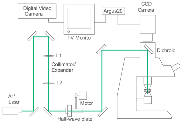
FIG. 1. (Color online) Diagram of the optical layout of the optical tweezers. Rotation of the linearly polarized light by rotation of a half-wave plate applies a torque to the nanorods in the sample between the two objectives.
