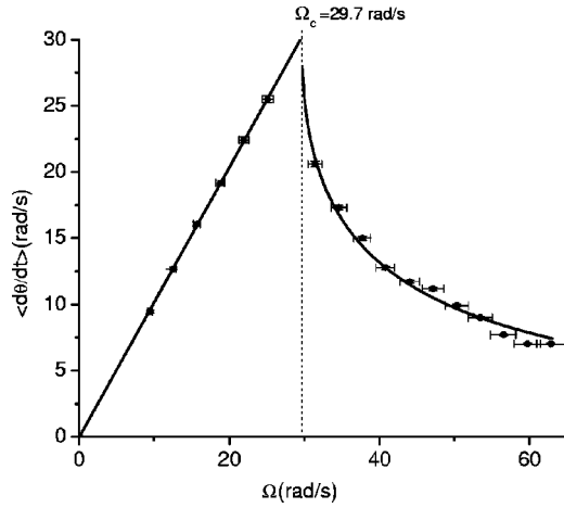
FIG. 9. Plot of the average nanorod rotation rate \langle d\theta/dt \rangle versus the laser-polarization-rotation rate \Omega . For values of \Omega < \Omega_c , the dependence is linear. For \Omega > \Omega_c , the rod rotation rate declines monotonically as \Omega is increased. In both regions, the solid curves represent the fitted function; for \Omega < \Omega_c , the function is linear and for \Omega > \Omega_c , the fitted function is given in Eq. (4). Vertical error bars are about 1% of the y values, while the horizontal error bars are 3% of x values.
