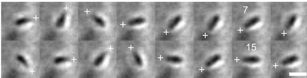
FIG. 5. A sequence of images showing the motion of a nanorod under the influence of the light torque with a nonphased response, i.e., the rod is not moving in phase with the rotating polarization of the light. The motion is counterclockwise from left to right, as indicated by the crosses (+) that follow one end of the nanorod for all 16 images. It is clear that the nanorod periodically reverses direction, as in frames 7 and 15 here. The angular polarization rotation rate was \Omega=2\pi\times 5 Hz. Scale bar corresponds to 4\ \mu\text{m} .
