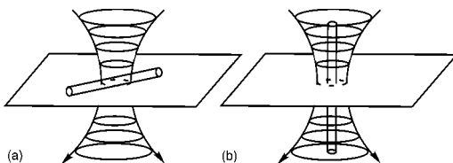
FIG. 2. A sketch of the orientations possible for nanorods described here. The nanorods are trapped in a focused Gaussian beam propagating down. In (a), the nanorod is transversely oriented with respect to the light propagation axis. In (b), the nanorod is axially oriented.
