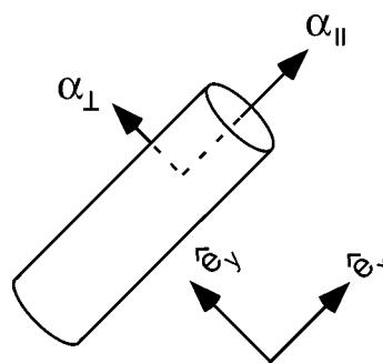
FIG. 10. Sketch showing the tensor components in the body frame of the rod.
