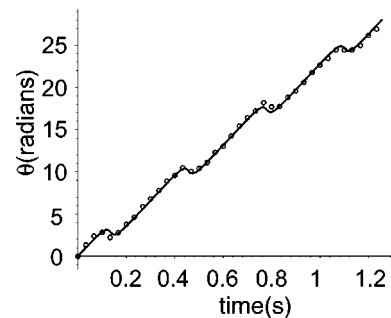
FIG. 8. A plot of the nanorod orientation \theta as a function of time t . The solid curve corresponds to a nonlinear least-squares fit to the data. The final values for the fitting parameters were \Omega=2\pi\times 5.14 Hz, \Omega_c=2\pi\times 4.90 Hz, and \beta=1.65 (see text for details).
