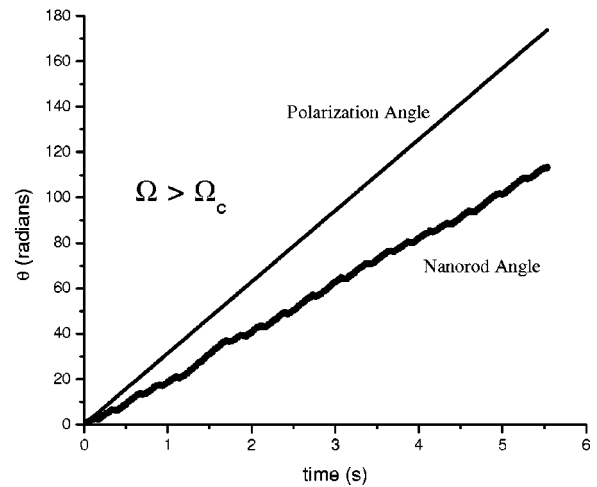
FIG. 7. A plot of the nanorod orientation \theta as a function of time t for nonlinear motion. In addition, we have plotted the laser polarization rotation angle \Omega t during the same time. This corresponds to the case where \Omega=2\pi\times 5 Hz and \Omega_c\approx 2\pi\times 4.8 Hz.
