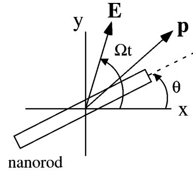
FIG. 3. A sketch of the light torque geometry. Here the induced dipole \mathbf{p} will move to align with the electric field \mathbf{E} to minimize energy. Hence, a torque \boldsymbol{\tau} = \mathbf{p} \times \mathbf{E} exists about an axis out of the plane of the paper. The light propagation direction is into the paper.
