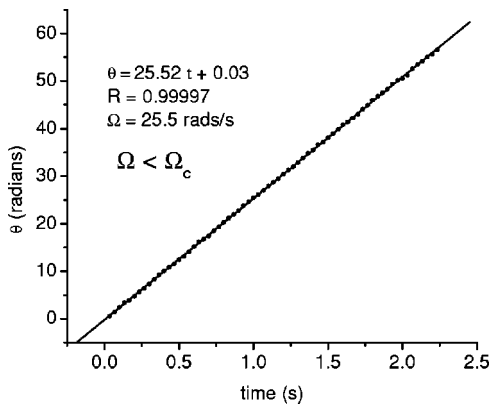
FIG. 6. A plot of the nanorod orientation \theta as a function of time t for linear motion. Here \Omega=2\pi\times 4.06 Hz and \Omega_c\approx 2\pi\times 4.8 Hz, so \Omega < \Omega_c . The solid line represents the best linear fit to the data.
